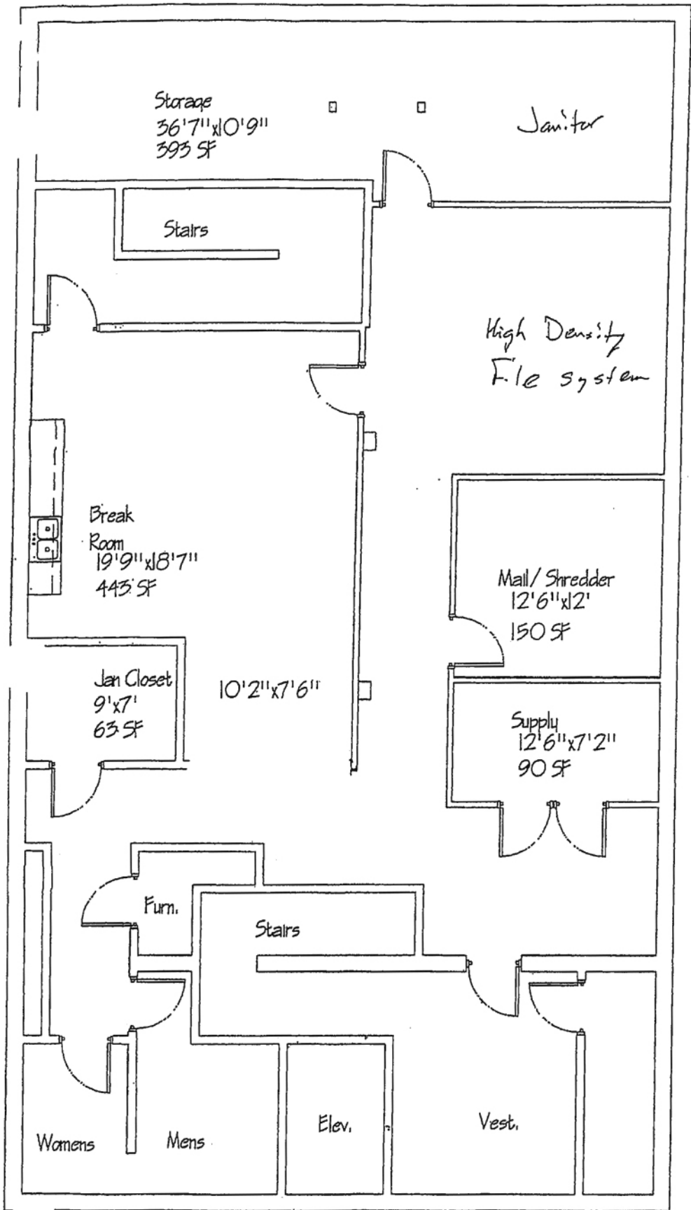
BASEMENT FLOOR
