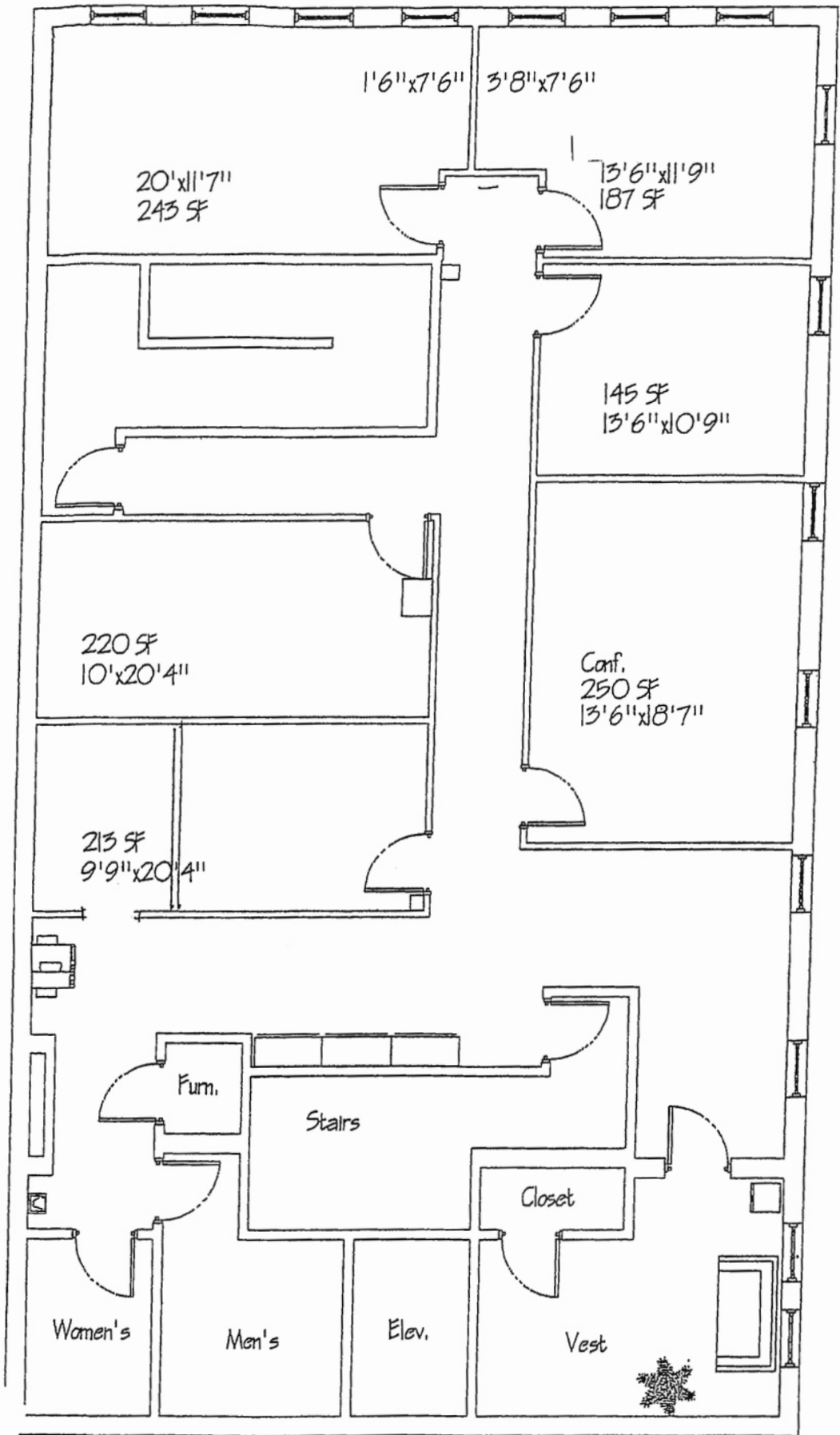
SECOND FLOOR
